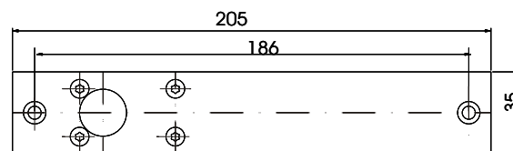
Face plate
