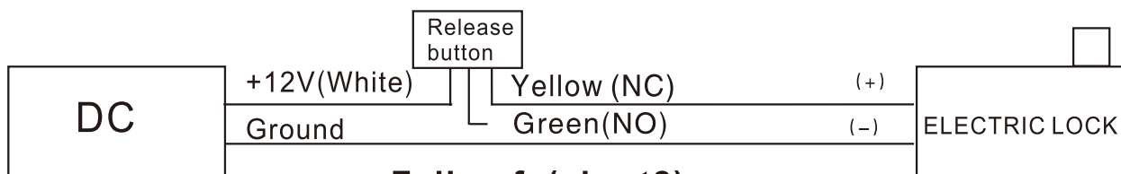
Fail-safe(chart2)
