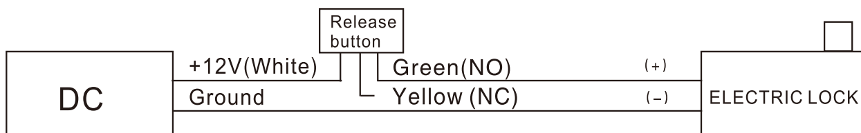
Fail-secure(chart1)
