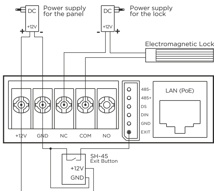
Connection scheme of electromagnetic lock using external power supply for panel and the lock.
